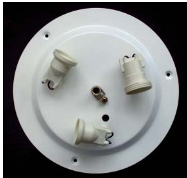
20 275 00 Deckenhalter, E 27, dreiflammig Ceiling fixture, E 27, 3 - light Ø 30 cm
