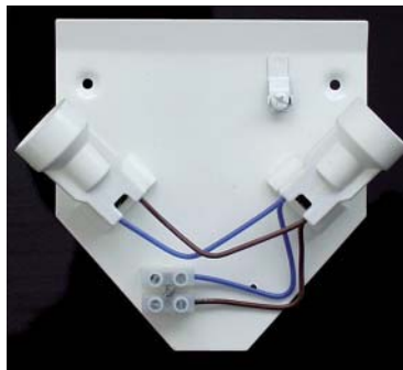
20 261 00 Wandhalter, E 14, zweiflammig Wall fixture, E 14, 2 - light
